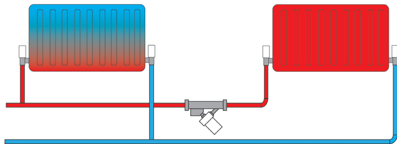
Diagram 14.2 Shows an original SPB radiator flow booster boosting a single radiator
