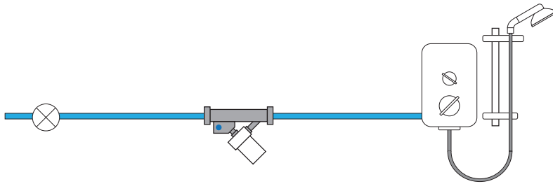
Diagram 14.1 Automatic Pump (SP2B) installed on Mains fed cold to an Electric Shower.
